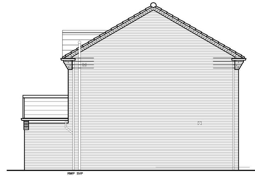
SIDE ELEVATION Alderton
