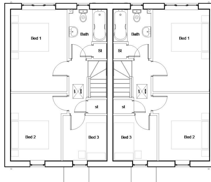
First floor Bamburgh Bamburgh
