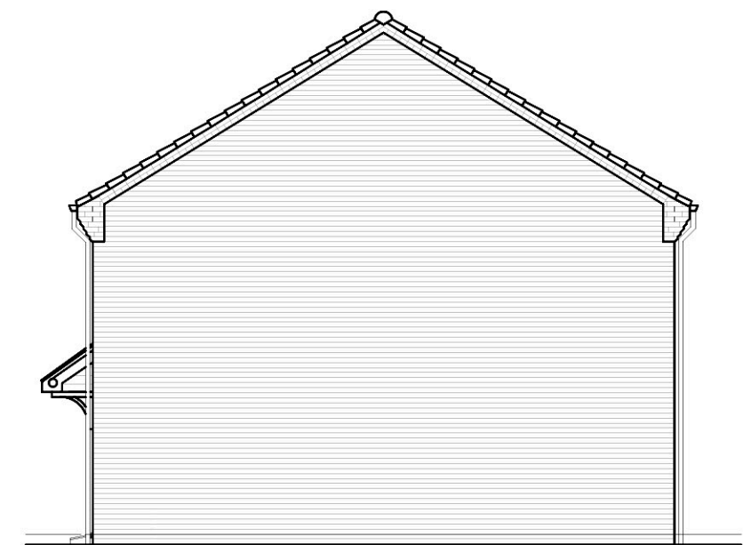
Side Elevation Bamburgh
