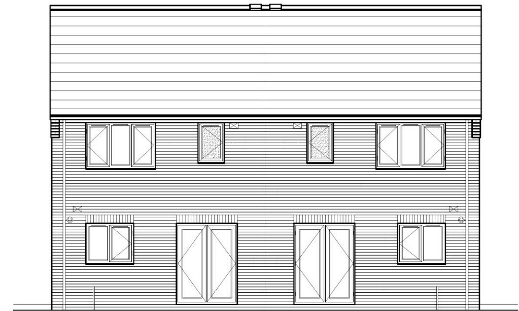
Rear Elevation Bamburgh Bamburgh
