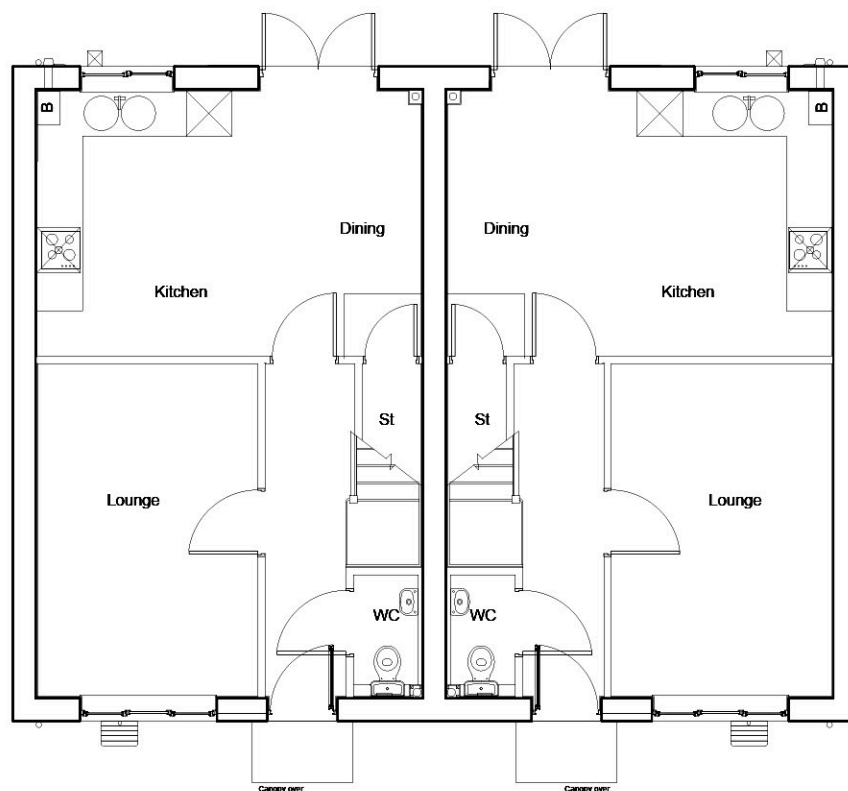
Ground floor Bamburgh Bamburgh
