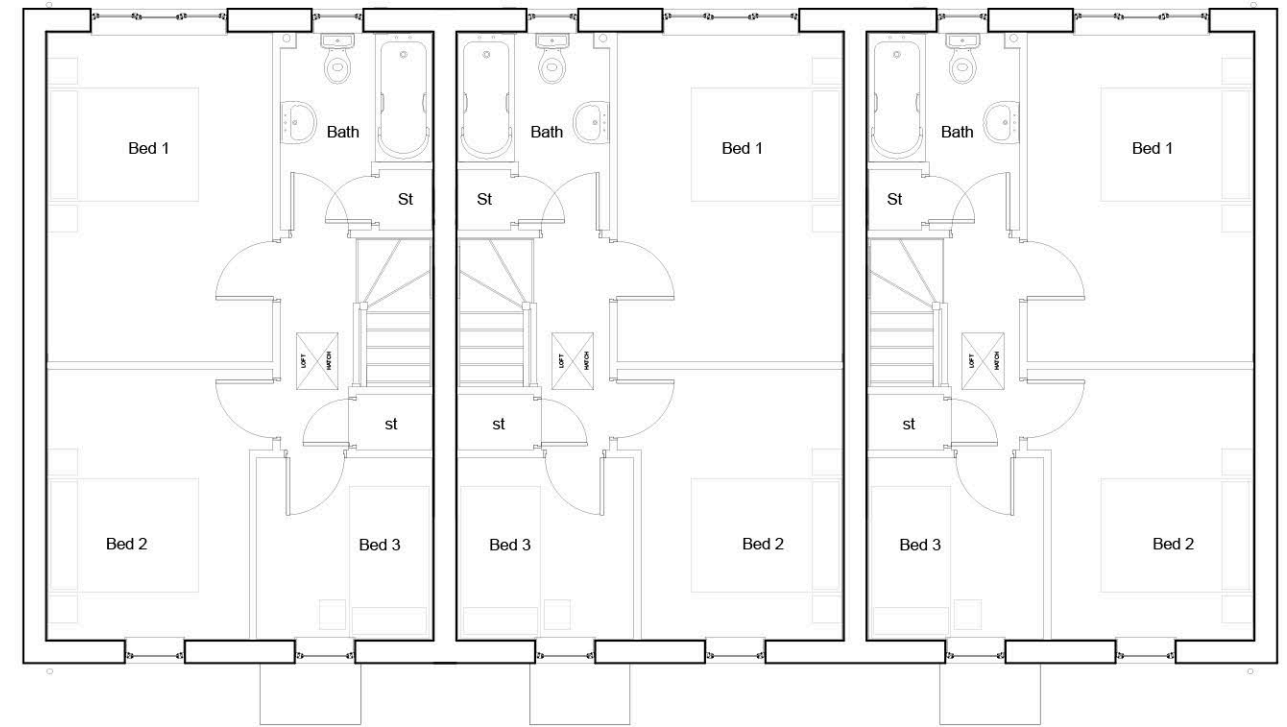
First floor Bamburgh Bamburgh Bamburgh
