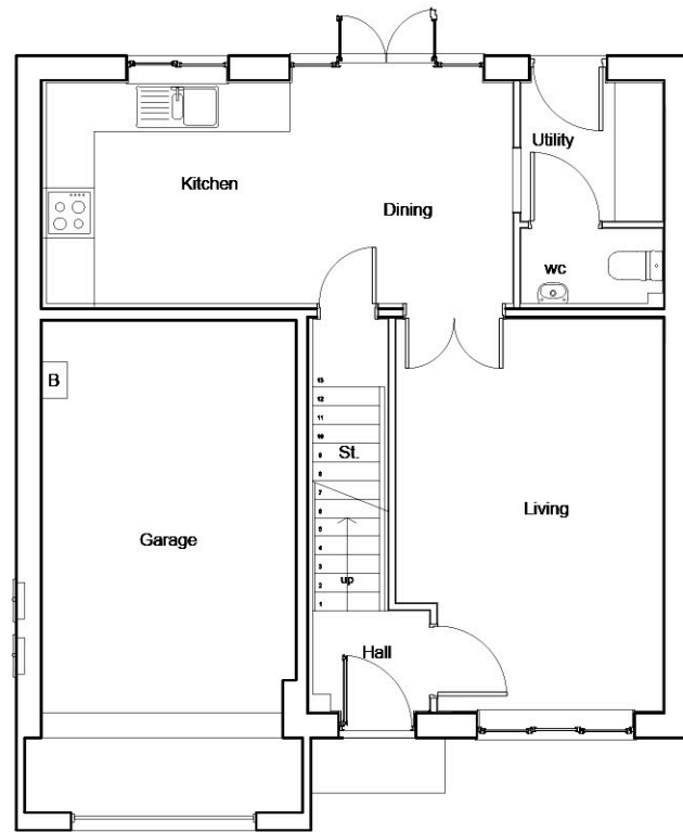
Baybridge GROUND FLOOR PLAN
