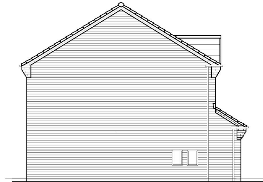
Baybridge SIDE ELEVATION
