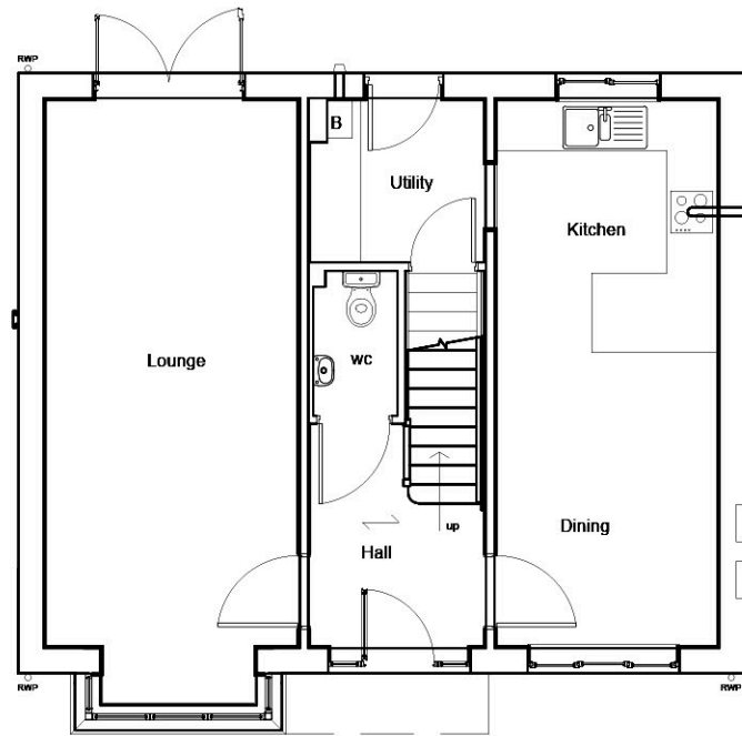
GROUND FLOOR LAYOUT Grassington
