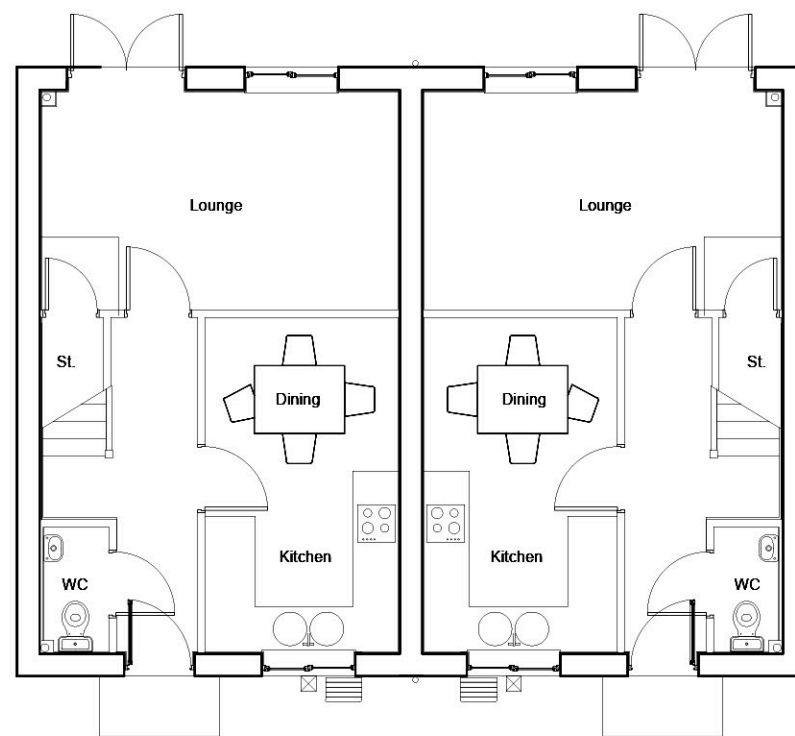
Ground floor Hadleigh
