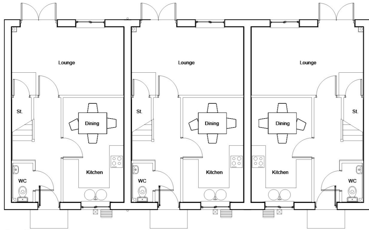
Ground floor Hadleigh Hadleigh Hadleigh
