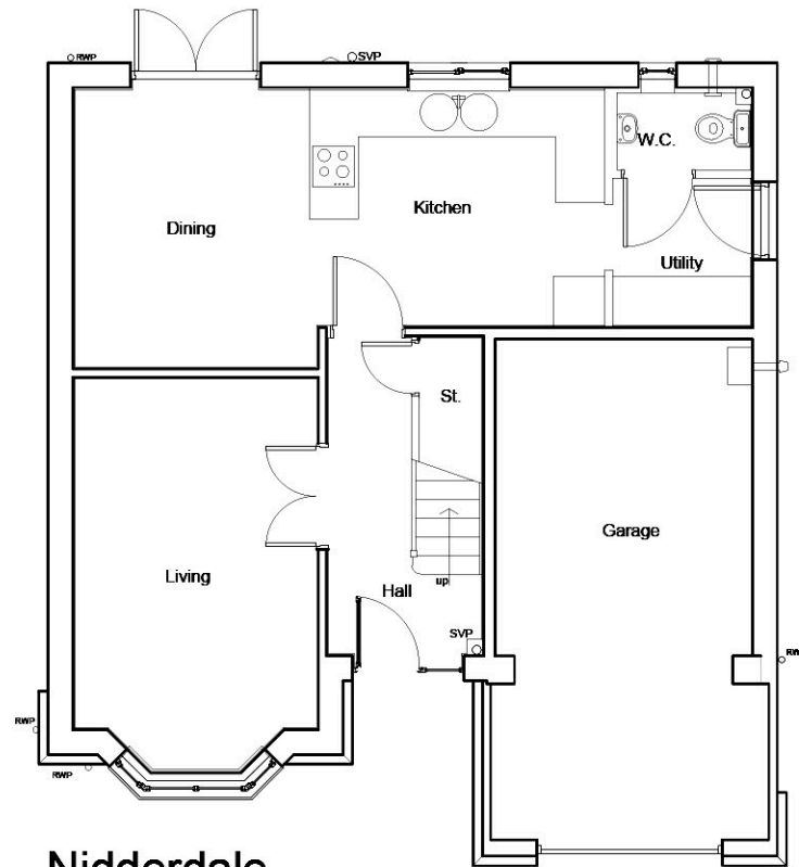
Nidderdale GROUND FLOOR PLAN
