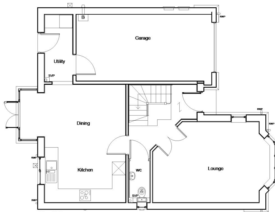
Settle FIRST FLOOR PLAN
